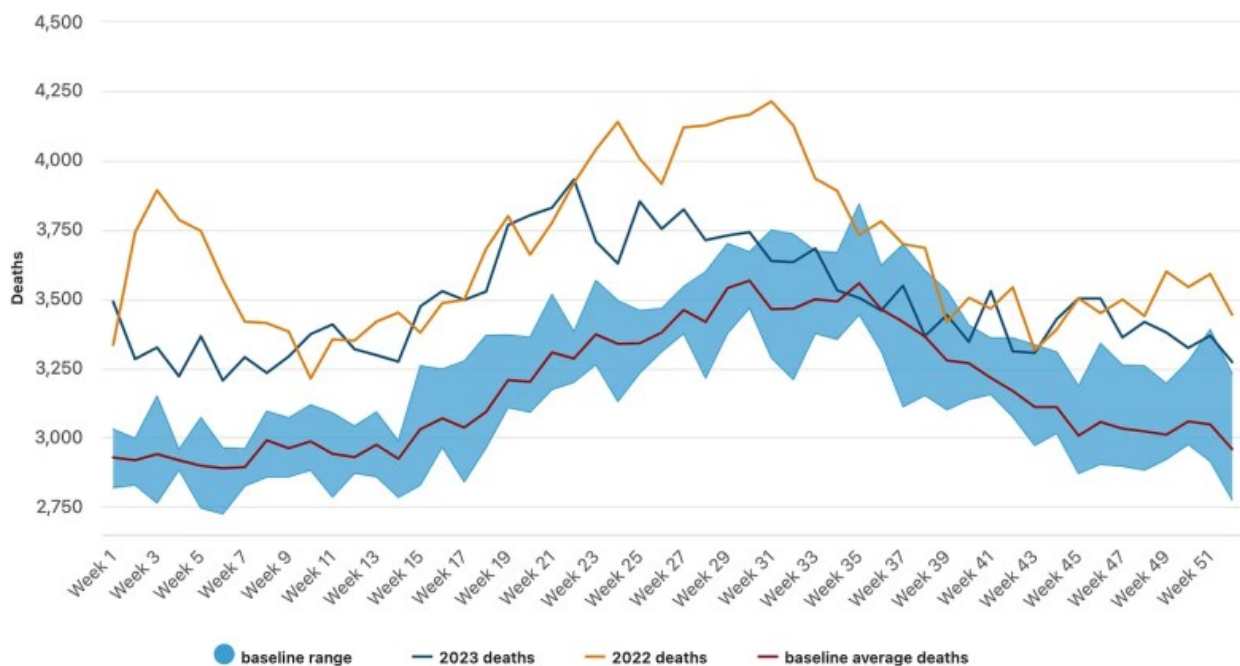
All deaths, Australia, 3 January 2022 - 31 December 2023 vs baseline benchmarks
