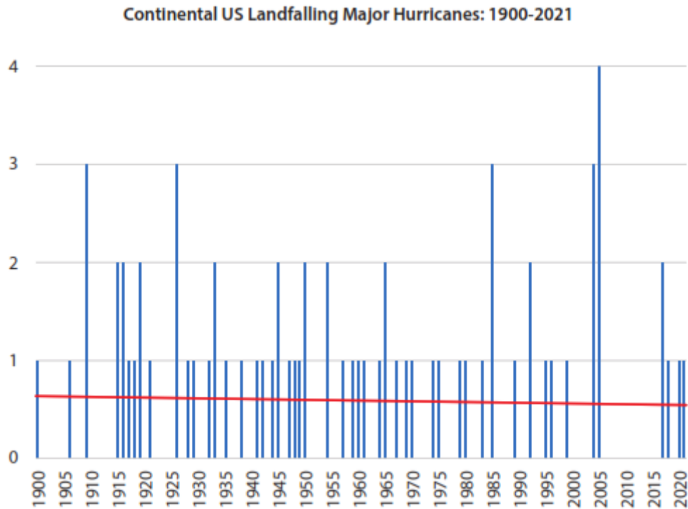
Figure 3. Number of major continental US landfalling hurricanes. This graph was updated from Klozbach 2018 by Roger Pielke Jr. The illustration is from Crok and May 2023.
