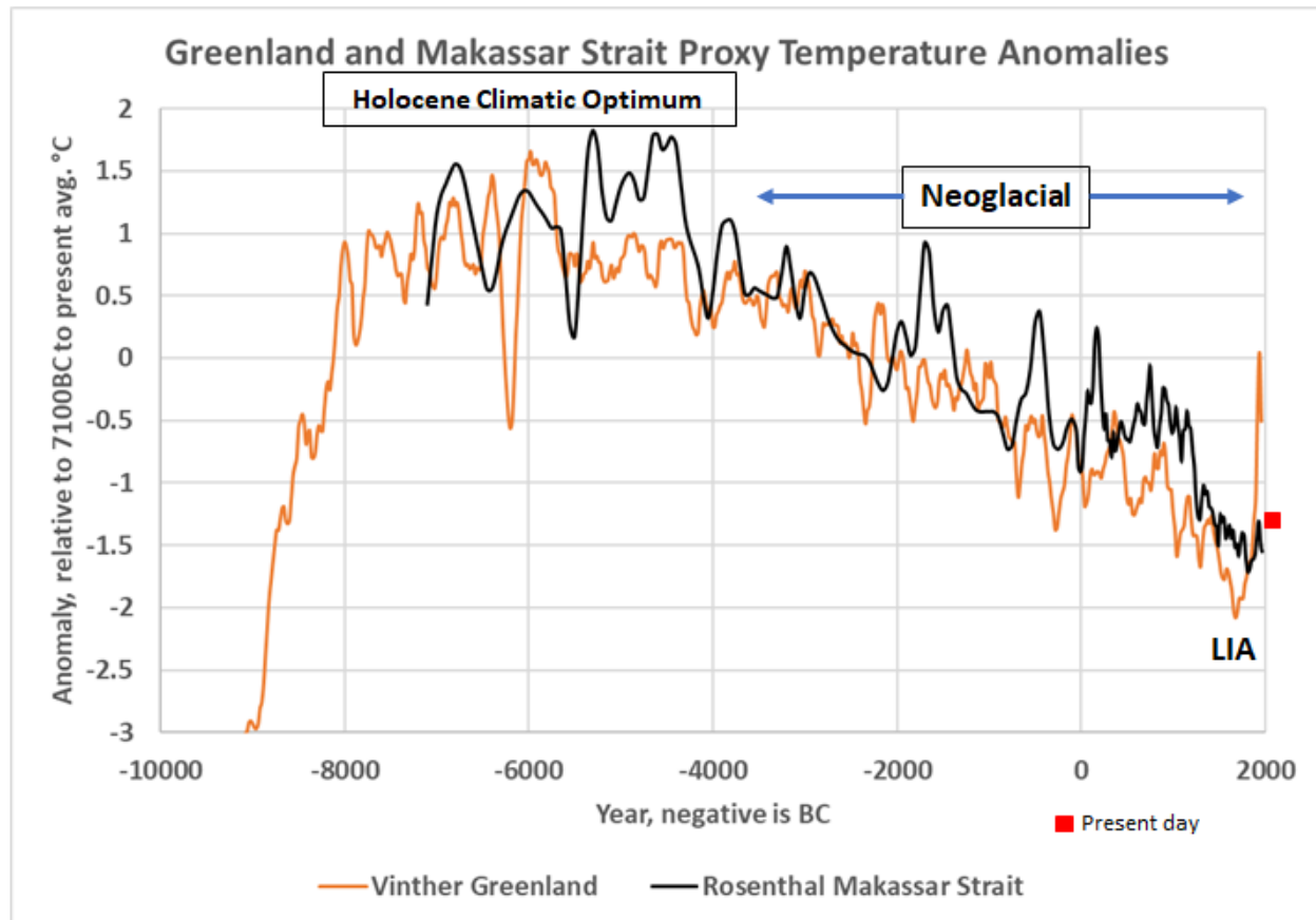
Figure 4: Greenland ice core (Vinther, et al., 2009) and Makassar Strait, Indonesia intermediate water (500 meters) temperature proxy (Rosenthal, Linsley, & Oppo, 2013) anomalies since the Holocene Climatic Optimum. The present day average temperature anomaly in the Makassar Strait at 500 meters depth from 2006 to 2016 is marked with a red box.
