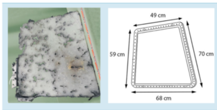
Figure 34: Left cockpit window 2. (Source: Dutch Safety Board)
