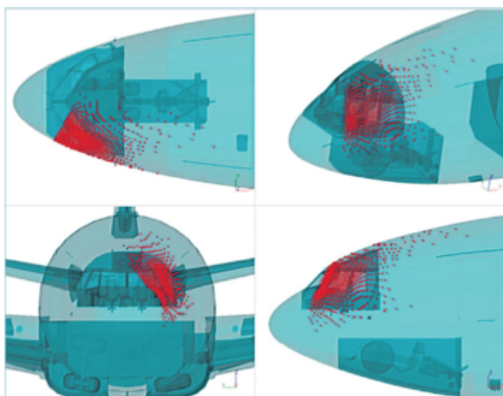
Figure 60: Image of the damage pattern produced by the model of a 40 kg warhead in the warhead simulation model. (Source: TNZ)
