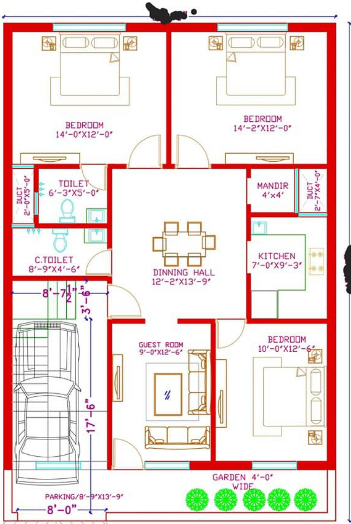
GROUND FLOOR
