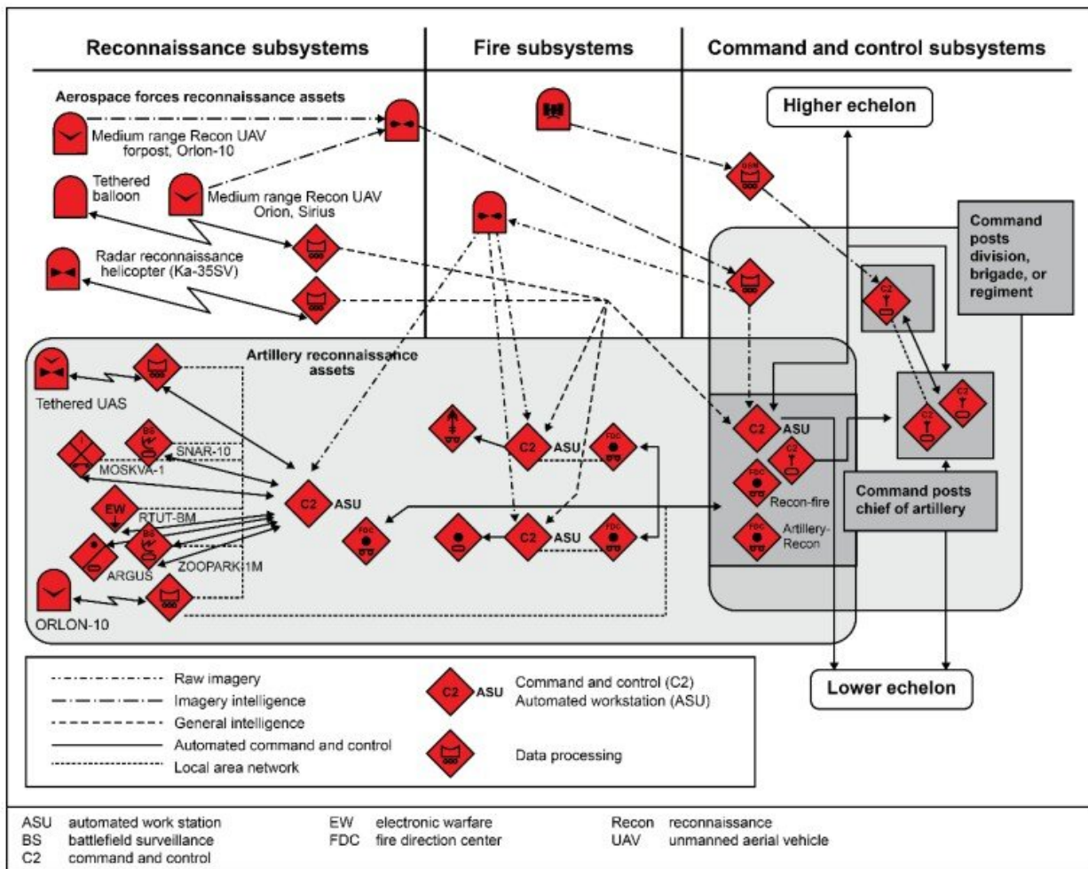
Figure 5-8. Fire control communication architecture
