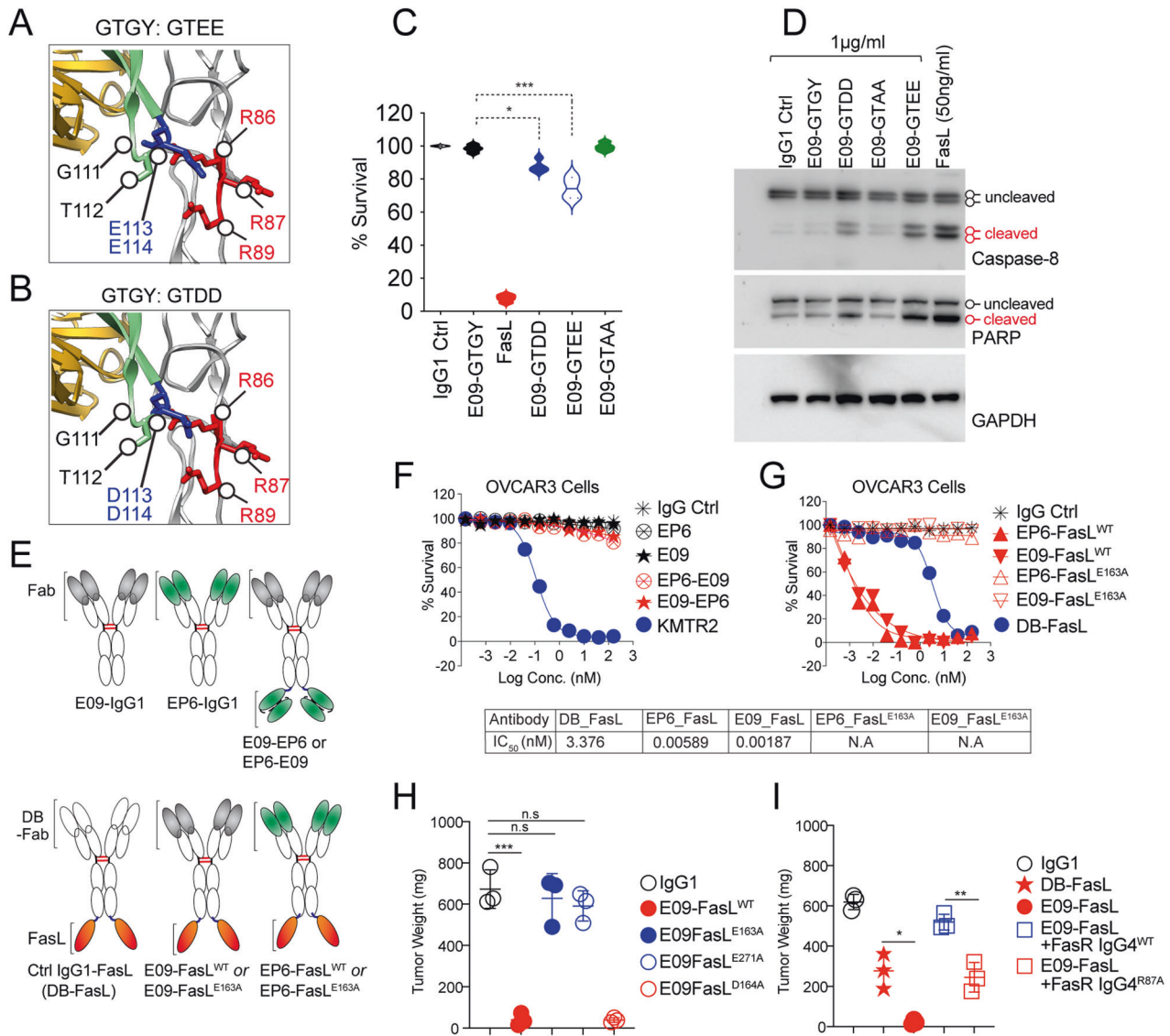
Fig. 7 Negative charge substitution in CRD3 of E09 VH partly restores its Fas agonist activity in tumor cells. A, B The zoomed-in structure of Fas ECD region in complex with E09 IgG1. The interface of the E09 Fab against Fas PPCR is highlighted (PDB:3TJE). VH (green), VL (gold), and Fas (gray) are as depicted as ribbons. WT E09 contains GTGY (green sticks) in the CDR3 loop (see Supplementary Fig. 6). GTGY residues of the CRD3 loop were mutated to GTEE or GTDD at 111–114 positions for the experiments described in (C) and (D) . C 0.5 µg/ml WT E09 IgG1 (GTGY) or E09 IgG1 (GTEE or GTDD or GTAA) at 111–114 positions of E09 VH CRD3 along with other controls were added onto OVCAR3 in cell survival analysis post 36 h ( n = 3+ ). D Same as (C) , except indicated molecules (FasL at 20-fold lower concentration) were added for 10 hrs, followed by immunoblotting for caspase-8 and PARP. E Schematic showing genetic construction of generation of Fas agonist (E09, EP6) bispecific antibodies and antibody ligand bispecific combinations. F A 96-well plate OVCAR3 cell killing assay of indicated E09, EP6 Fas agonist monospecific antibodies, and E09-EP6 combination bispecific antibodies. KMTR2 was used as a positive control of killing. G Same as (F) , except E09-FasL and EP6-FasL bispecific combinations were used with FasL WT or FasL E163A . IC 50 values are shown ( n = 3 ). H 1 \times 10^6 – 1.5 \times 10^6 OVCAR3 tumor cells were injected subcutaneously in NOD.Cg-Prkdc scid I12rg tm1Wjl /SzJ animals with Matrigel in PBS. When tumors appeared on animals (3–4 weeks), animals were i.p. injected with indicated E09-FasL bispecific combinations either with FasL WT or FasL E163A or FasL D164A or FasL E271A ( n = 3+ ). I Same as (H) , except 4-fold recombinant Fas-IgG4 WT and Fas-IgG4 R87A proteins were co-injected in indicated cases along with E09-FasL ( n = 3+ ). Error bars in (H) and (I) represent SEM ( n = 3+ ).
