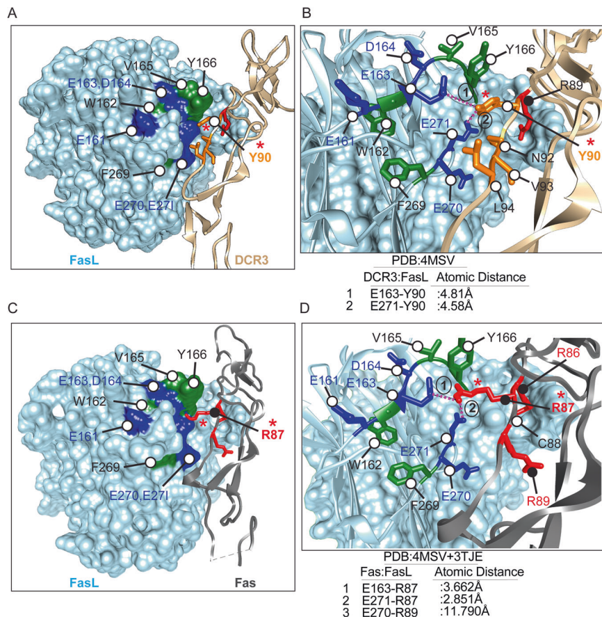
Fig. 2 FasL forms salt bridges with Fas R87 residue. A A space-filling representation of FasL surface (sky blue) at the interface of PPCR corresponding region of DCR3 (gold color shown as ribbon structure). Blue and green surfaces in FasL highlight the negatively charged and hydrophobic residues, respectively. Fas PPCR corresponding residues of DCR3 are shown in red and orange sticks. B Zoomed interface of FasL and DCR3 at PPCR from (A). Y90 (orange stick near red asterisk) of DCR3 acts like a “key” to insert itself into hydrophobically stabilized “lock” of negatively charged residues (E163, E271). Additional hydrophobic residues of DCR3 at its Fas PPCR corresponding region are shown in orange. C Same as (A), except Fas (Gray ribbon) is overlaid instead of DCR3. Fas PPCR residues are shown in red sticks. D Zoomed interface of FasL and Fas at PPCR. Instead of tyrosine (Y90) in DCR3, R87 (red stick near red asterisk) of Fas form significantly close salt-bridges (3.66 and 2.85 Å) with FasL negatively charged residues E163 and E271. The guanidine side chains of R86 and R89 are oriented away from the FasL PPCR interface motif.
